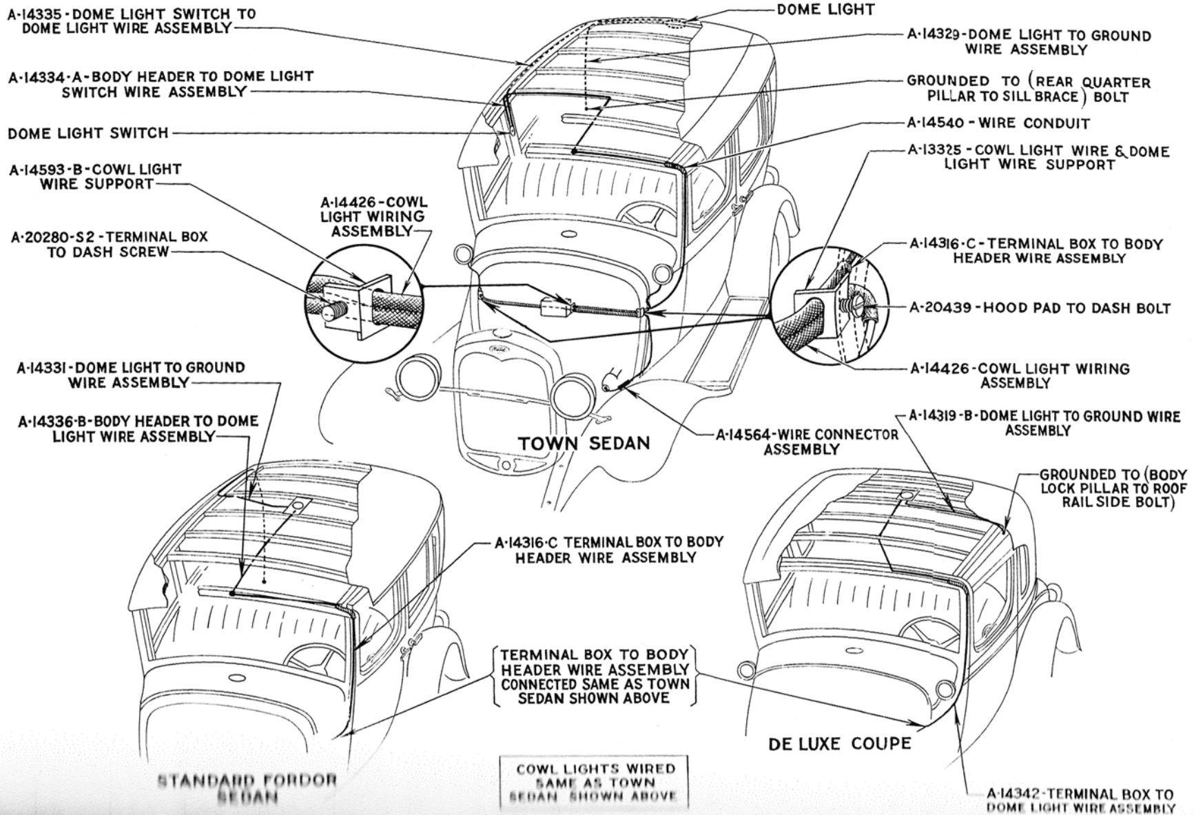
Fig. 838 - Wiring Diagram of Town Sedan, Standard Fordor Sedan and De Luxe Coupe
